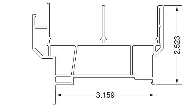
1b SL1101S HORIZONTAL ROLLER FRAME WITH FLANGE 0.079" EXT. WALL THK. 0.060" INT. WALL THK.
