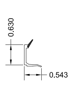
2 BV18 GLAZING BEAD 0.059" WALL THK.
