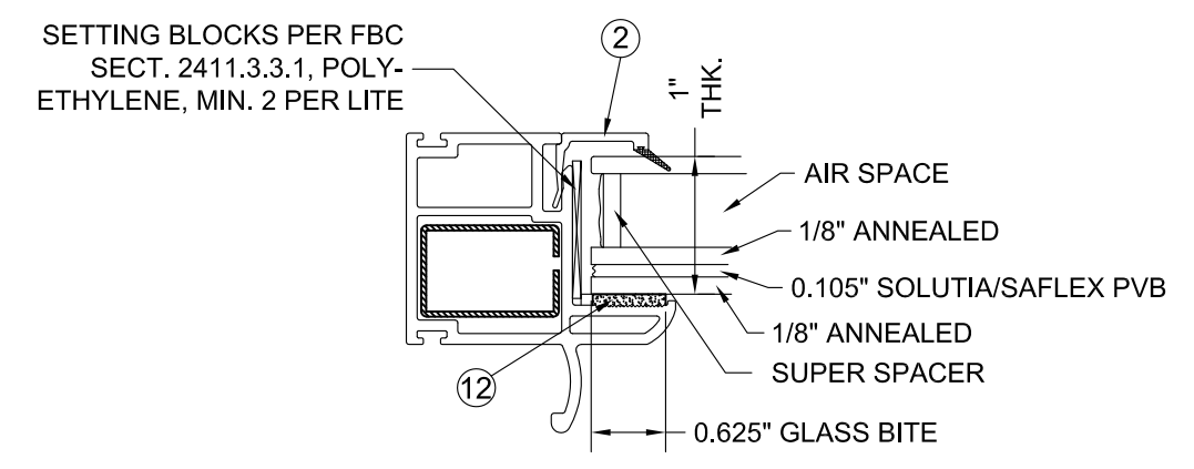
GLAZING DETAIL WITH SOLUTIA/SAFLEX LAMINATE
