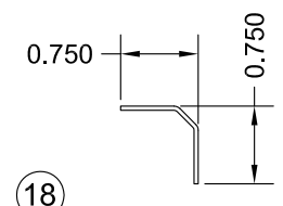
18 CM0220 ALUMINUM HEAD SUPPORT
