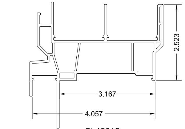
1c SL1201S HORIZONTAL ROLLER FRAME WITH NAILING FIN & J-CANNEL 0.079" EXT. WALL THK. 0.060" INT. WALL THK.
